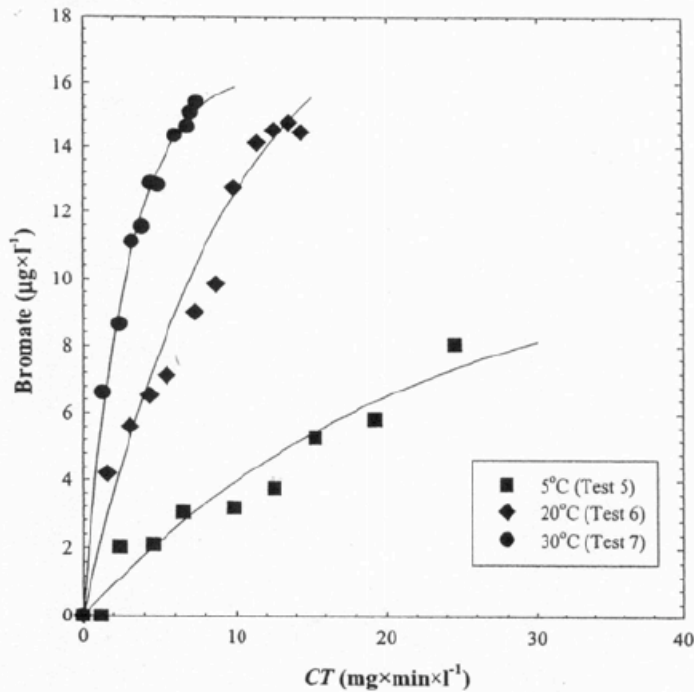
Fig.7 Bromate formation as a function of temperature in Lake Zürich water at pH 7. [Br] 0 = 33 µg/L. Adapted from Driedger et al. (2001).
