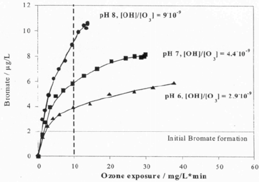
Fig.6 Bromate formation as a function of the ozone exposure for the pH range 6 – 8. [ experiments were performed in river Seine water spiked to a bromide concentration of µg/L. U. V. Gunten, 2001
